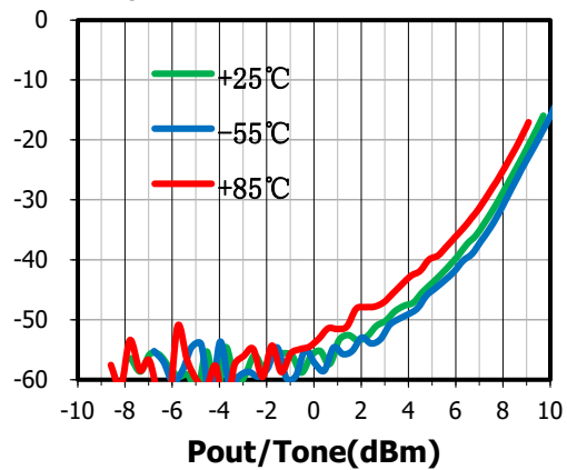
IM3(dBc)vs.Pout/Tone,f=9GHz
